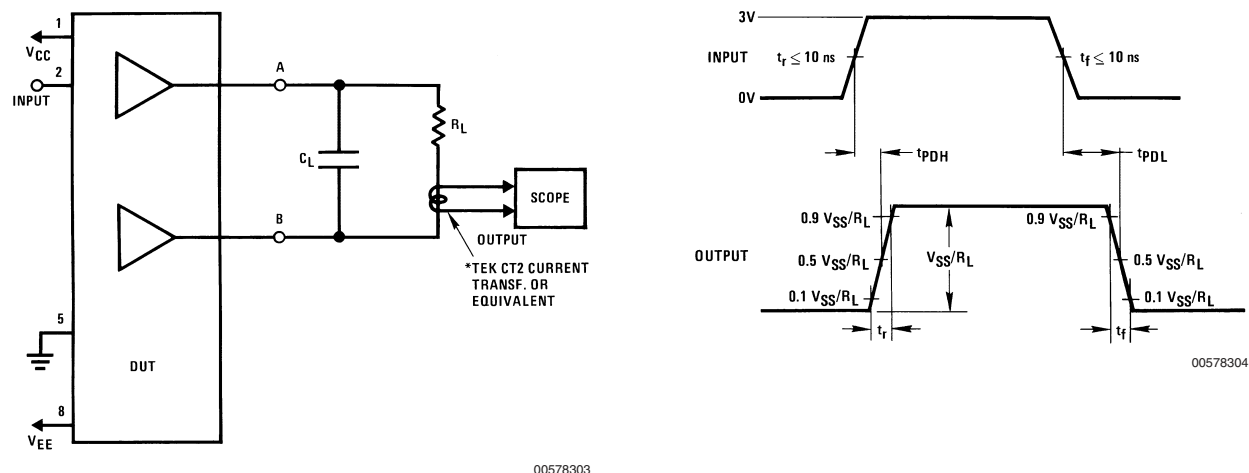
FIGURE 1. Differential Connection
