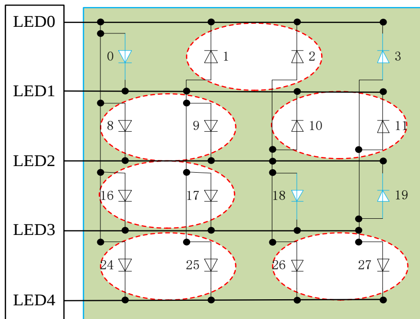
LED 4*4 点阵图
