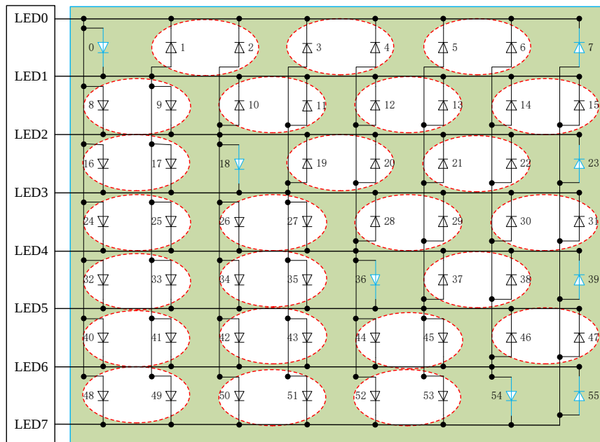
LED 7*8 点阵图
