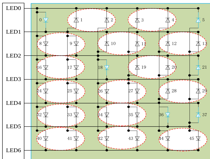
LED 6*6 点阵图
