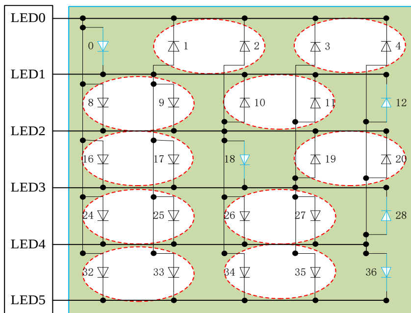
LED 5*5 点阵图
