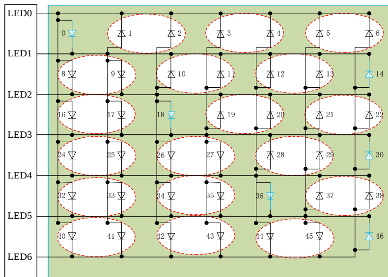
LED 6*7 点阵图
