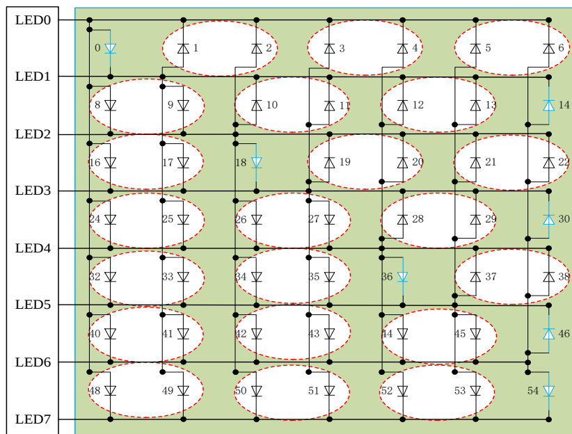
LED 7*7 点阵图
