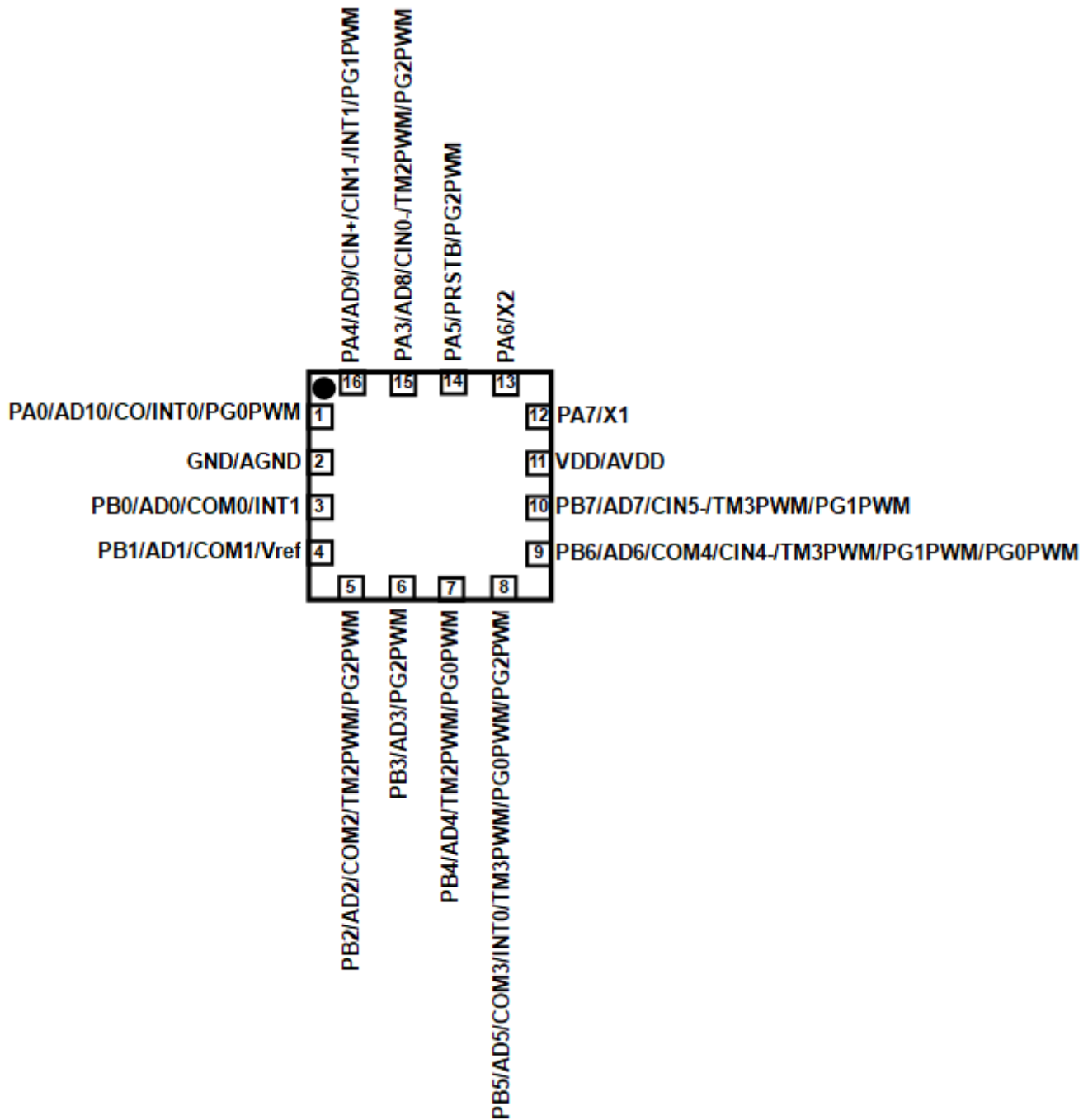
PFS123-1J16A (QFN3*3-16P-0.5pitch)
