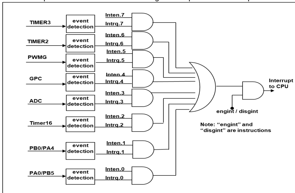
Fig.20: Hardware diagram of interrupt controller
