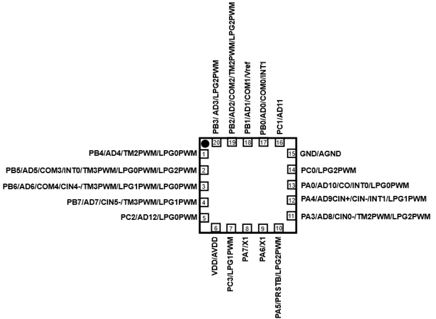
PFS123-1J20A(QFN3*3-20P)
