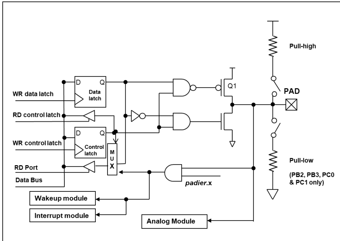
Fig. 21: Hardware diagram of IO buffer
