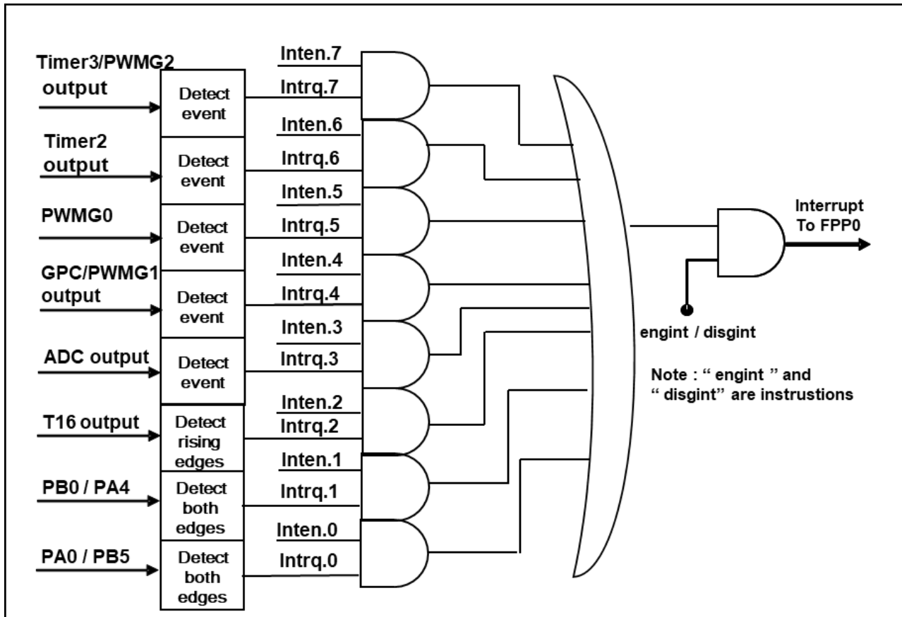
Fig.18: Hardware diagram of interrupt controller
