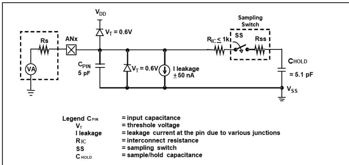
Fig.21: Analog Input Model
