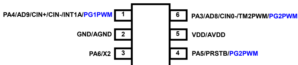
PMS132/PMS132B-U06 (SOT23-6 60mil)
