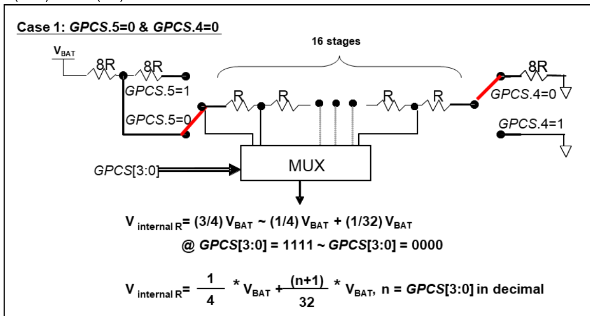
Fig.5: V_{\text{internal R}} hardware connection if \text{GPCS.5}=0 and \text{GPCS.4}=0
