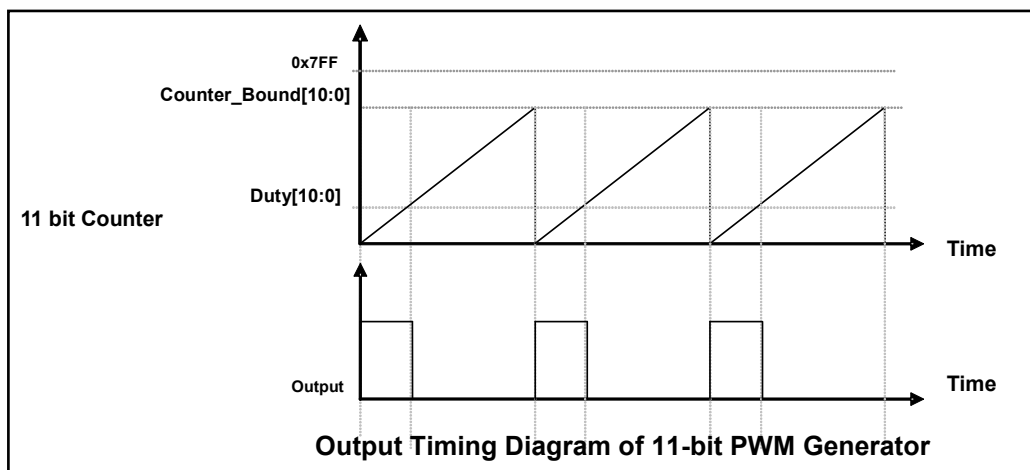
Fig.15: Output Timing Diagram of 11-bit PWM Generator
