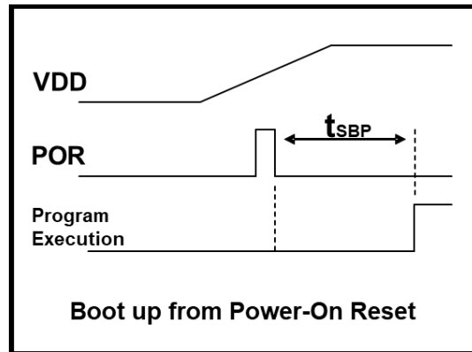
Fig.1: Power-Up Sequence
