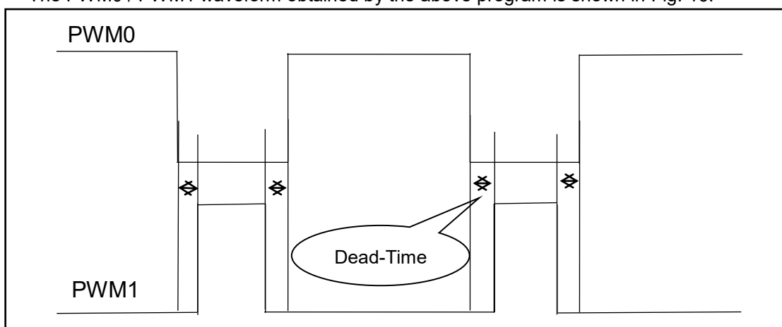
Fig. 16: Two complementary PWM waveforms with dead zones
