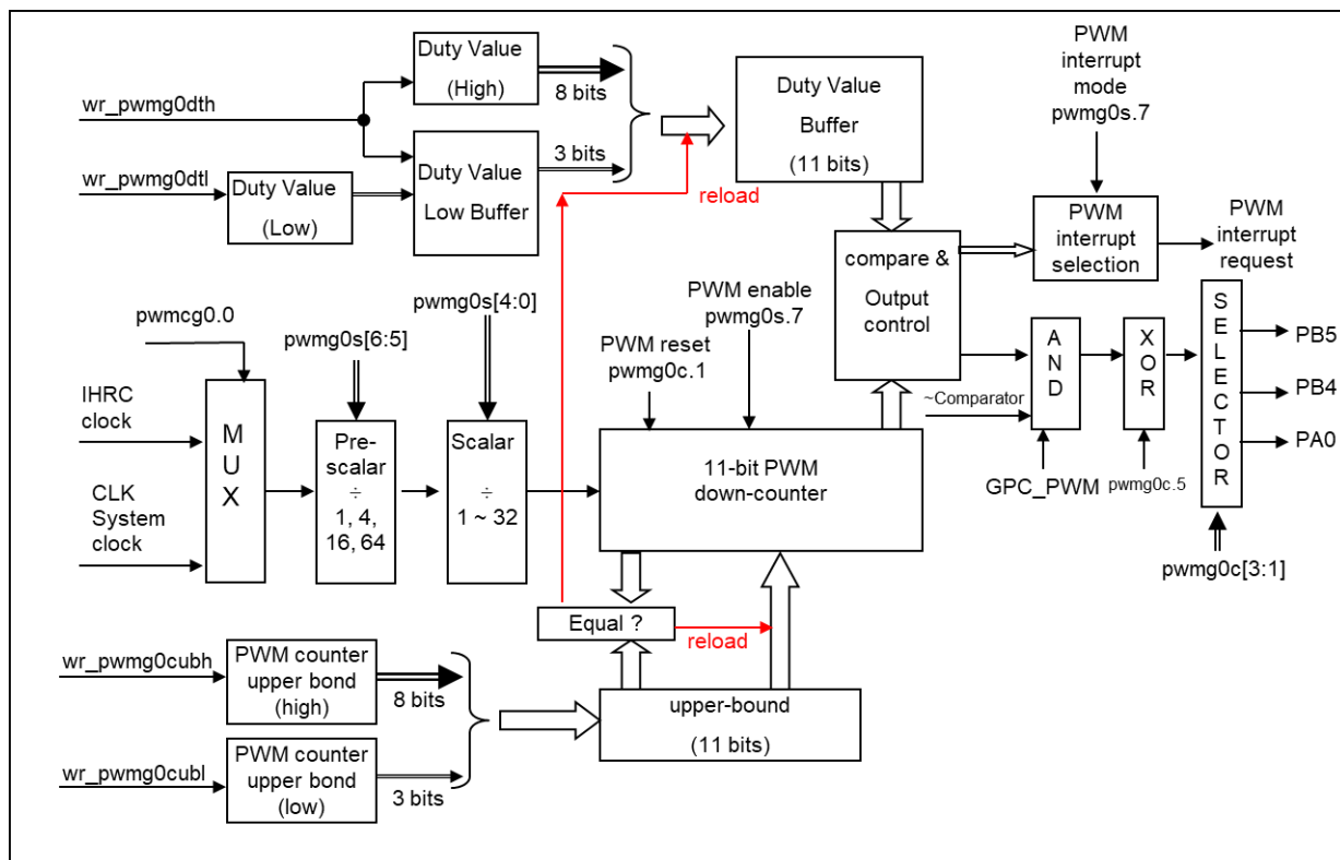
Fig.14: Hardware Diagram of 11-bit PWM Generator
