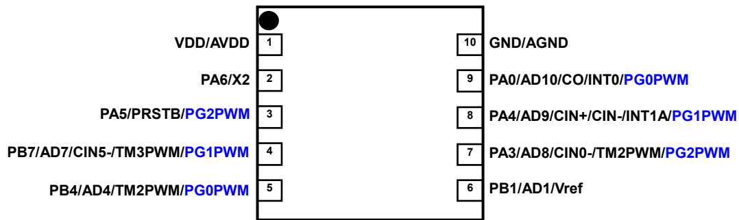
PMS132(B)-4N10 (DFN3*3-10P-0.5pitch)
