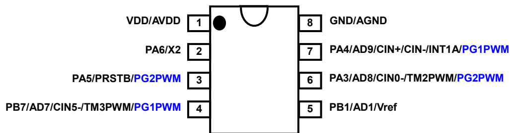
PMS132/PMS132B-S08 (SOP8-150mil)
