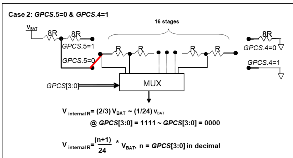
Fig.6: V_{\text{internal R}} hardware connection if \text{GPCS.5}=0 and \text{GPCS.4}=1
