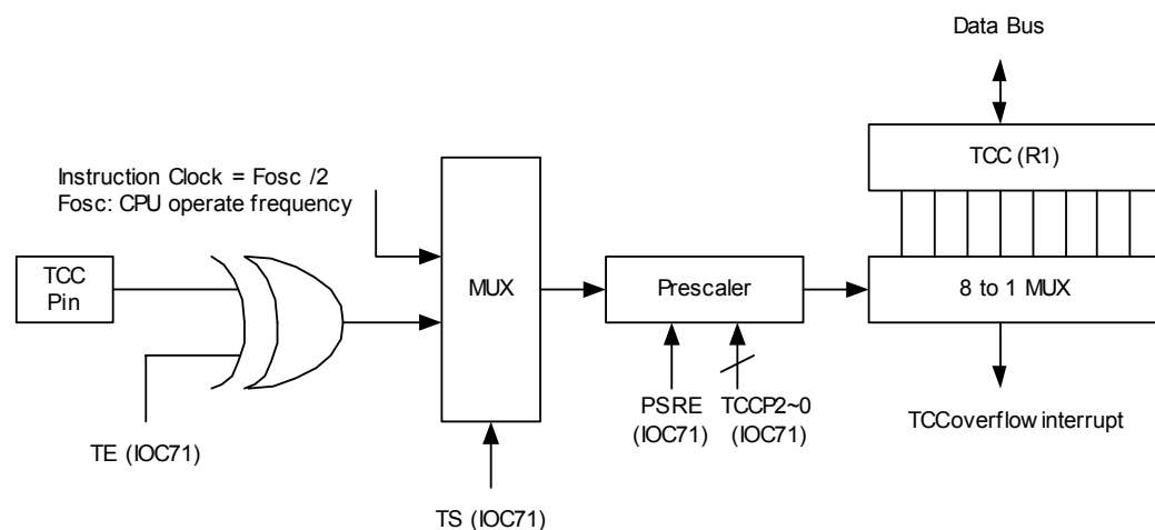
Fig. 7(a) Block Diagram of TCC
